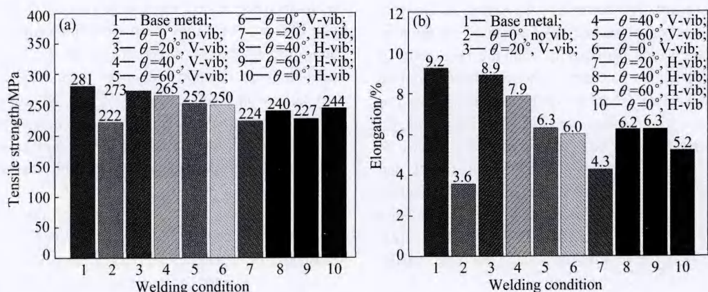
Fig. 10 Effect of vibrating parameters on tensile performance of weldments AZ31 sheet with thickness of 1 mm at 25%A: (a) Tensile strength; (b) Elongation
