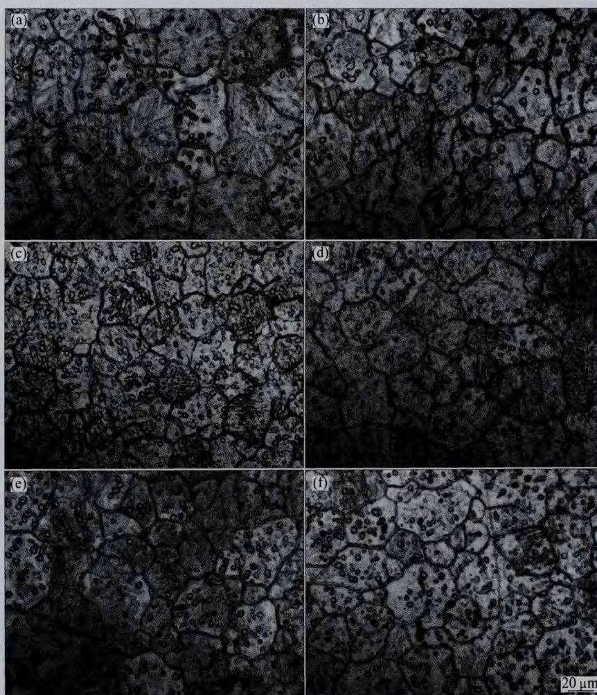
Fig. 5 Microstructures of TIG welded joints of AZ31 sheet with different vibration amplitudes, t=1 mm: (a) No vibration; (b) V-vib, 12.5%A; (c) V-vib, 25%A; (d) V-vib, 37.5%A; (e) H-vib, 12.5%A; (f) H-vib, 37.5%A
