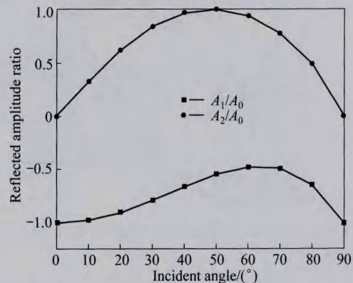
Fig. 7 Relative amplitude ratios A_1/A_0 and A_2/A_0 versus incident angles for AZ31 alloy
