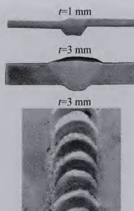
Fig. 3 Macro-morphology of vibratory welded seam
