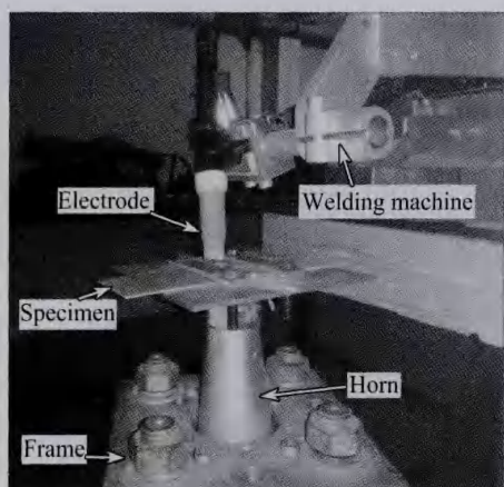
Fig. 2 Device for vibratory TIG welding
