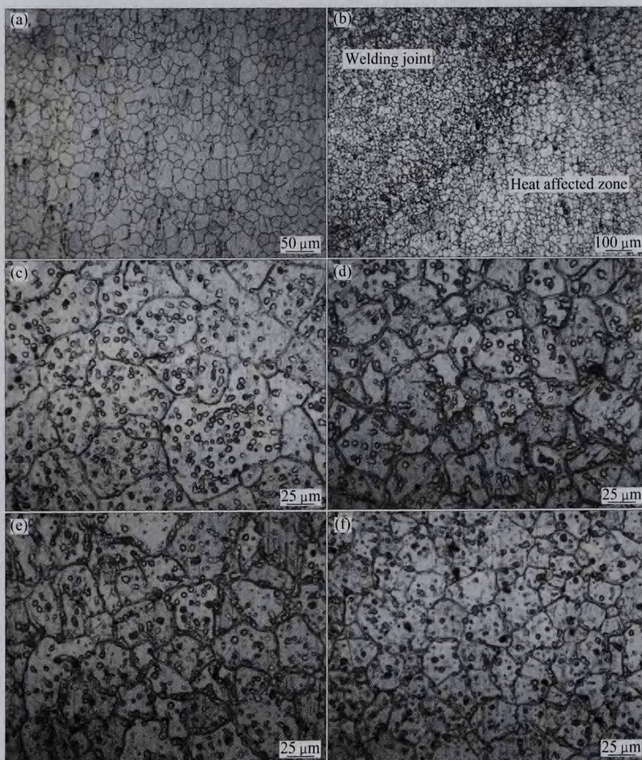
Fig. 4 Microstructures of base metal and joints welded with 25% vibration amplitude, t=3 mm: (a) Base metal; (b) V-vib, \theta=20^\circ , welding line border; (c) No vibration, \theta=0^\circ , welding line; (d) V-vib, \theta=0^\circ , welding line; (e) H-vib, \theta=0^\circ , welding line; (f) V-vib, \theta=40^\circ , welding line
