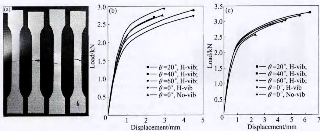
Fig. 9 Results of tensile test of TIG weldment under different conditions, t=1 mm and 25%A: (a) Tensile samples; (b) H-vib; (c) V-vib
