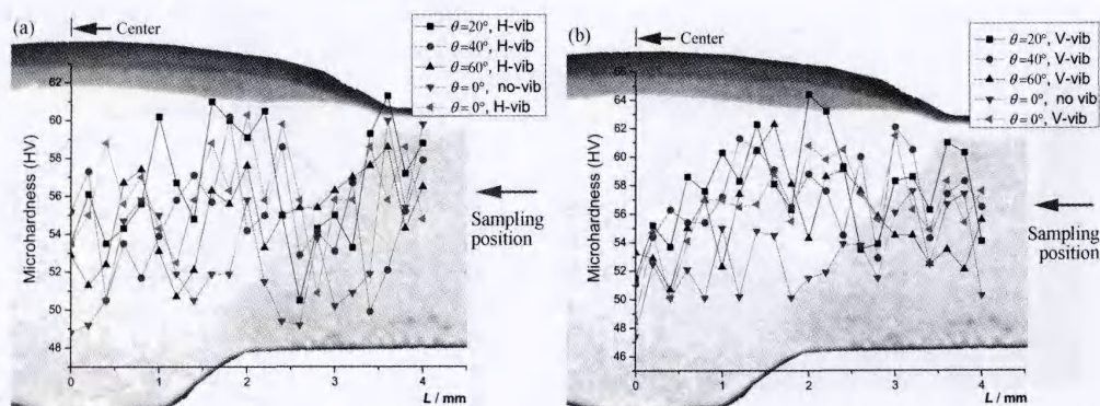
Fig. 8 Microhardness of TIG weld joints of AZ31 sheet with t=3 mm under different vibrating conditions and 25%A: (a) H-vib; (b) V-vib
