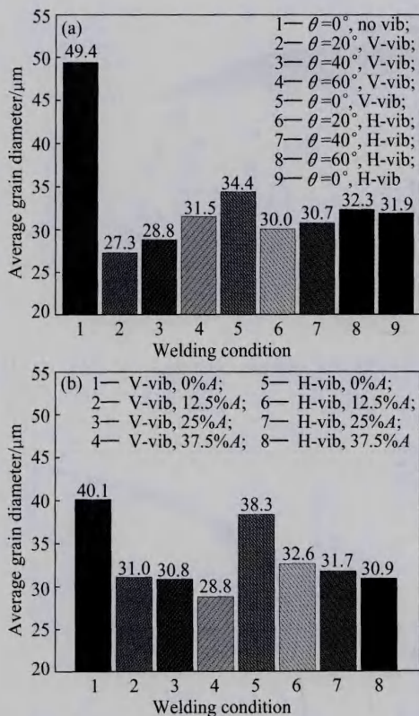
Fig. 6 Grain size of weld line under different welding conditions: (a) t=3\text{ mm} , 25%A; (b) t=1\text{ mm} , \theta=0
